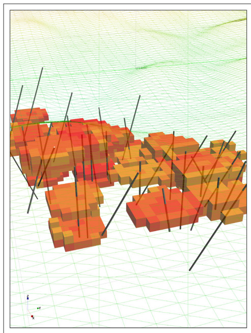
Area IV Block Model
