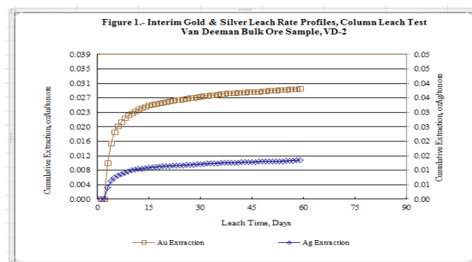
Gold recovery - 69.8% in 74 days of testing
